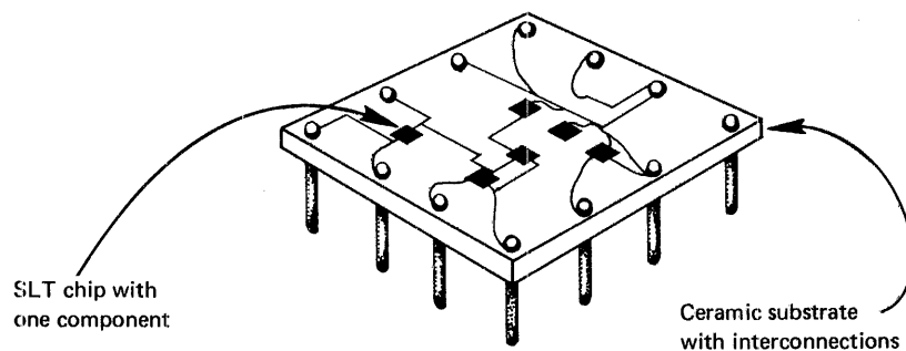
Figure 10.2. SLT substrate
