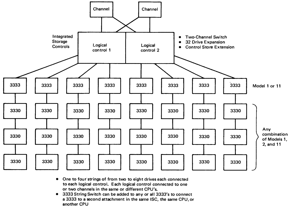
Figure 50.10.1. Permissible 3330-series string configurations for the Model 168 Integrated Storage Controls feature
