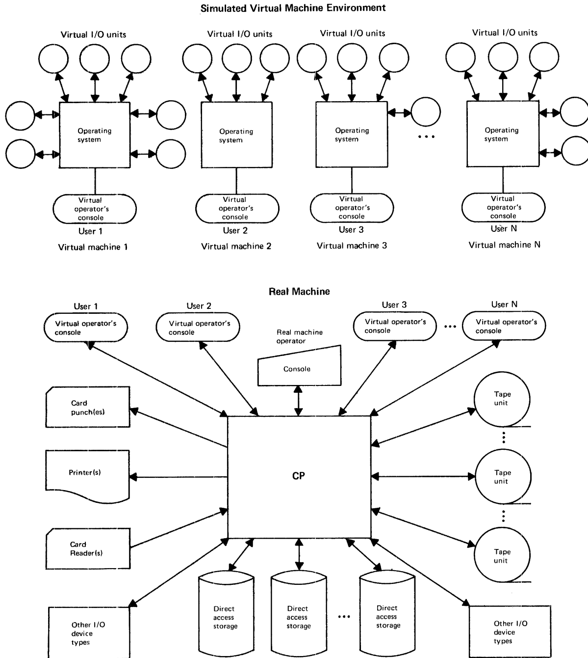
Figure 40.05.1. Conceptual illustration of the real and virtual machine environment that is supported by VM/370
