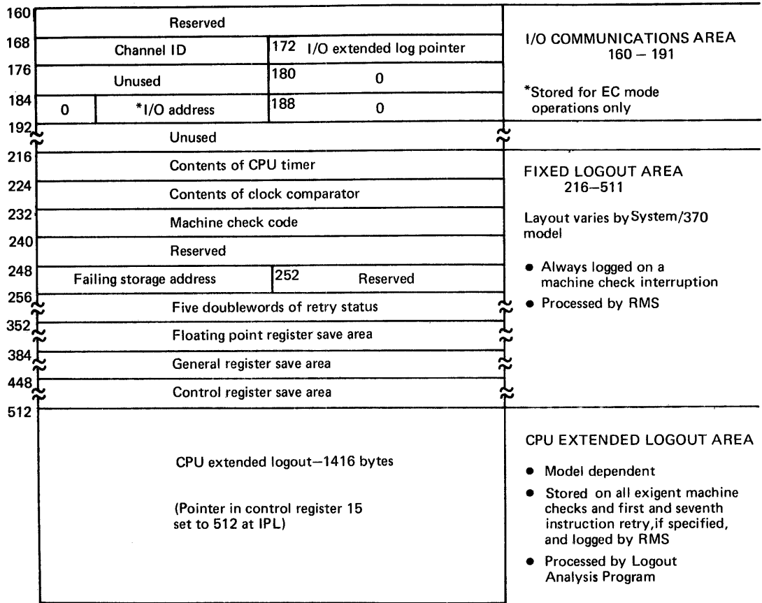
Figure 20.10.3. Model 168 (Model 1) model-dependent fixed storage locations
