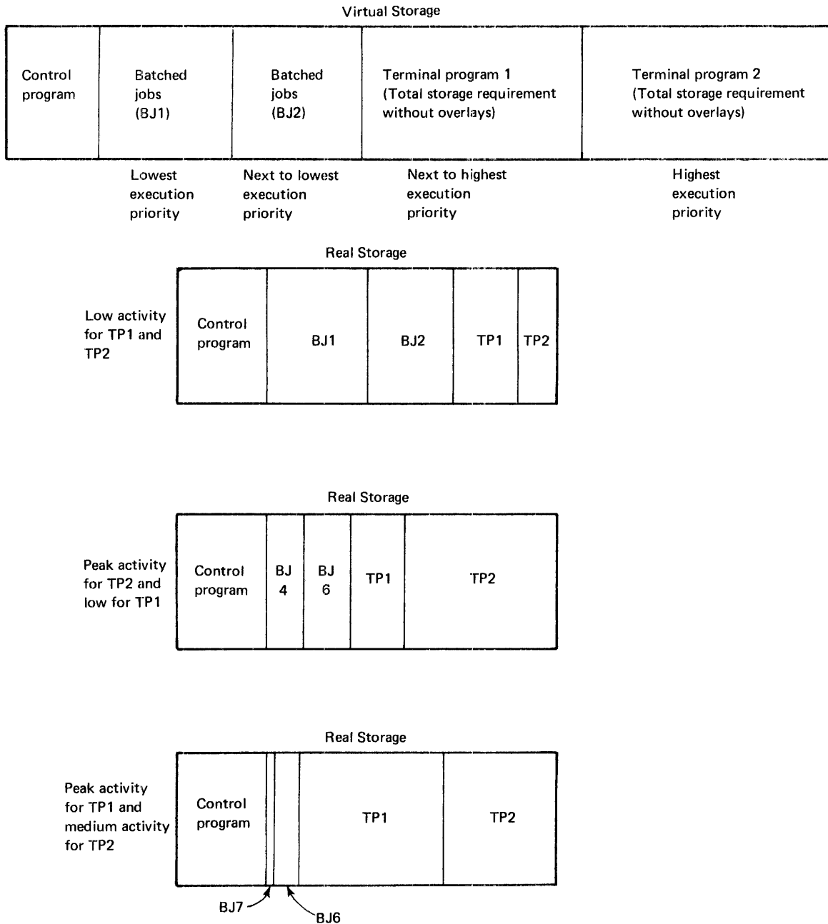
Figure 30.05.3. Conceptual illustration of real storage utilization in a mixed batch and online virtual storage environment
