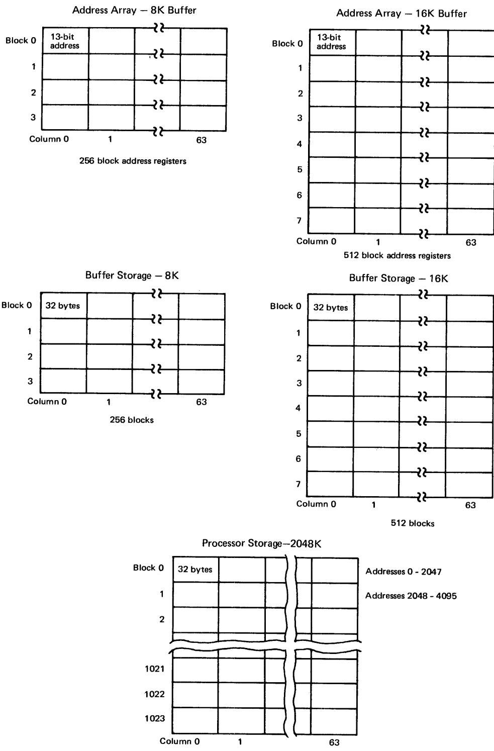
Figure 20.15.2. 8K and 16K buffer organization
