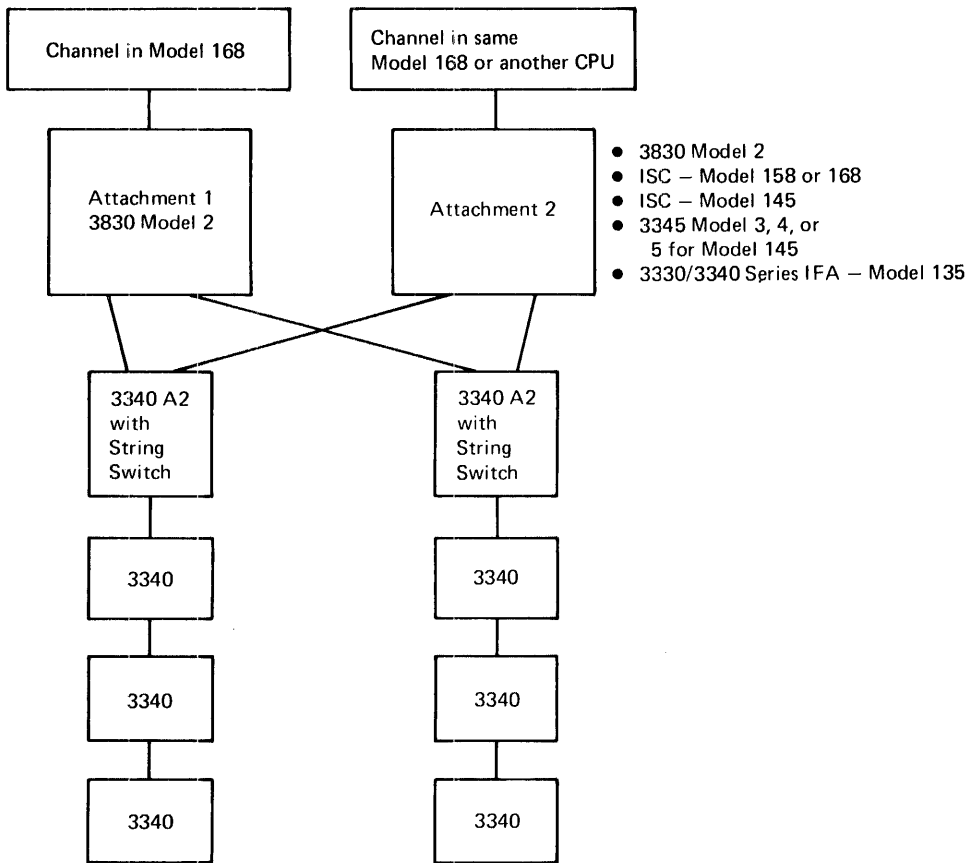
Figure 50.15.8. String switching for 3340 facilities attached to a 3830 Model 2
