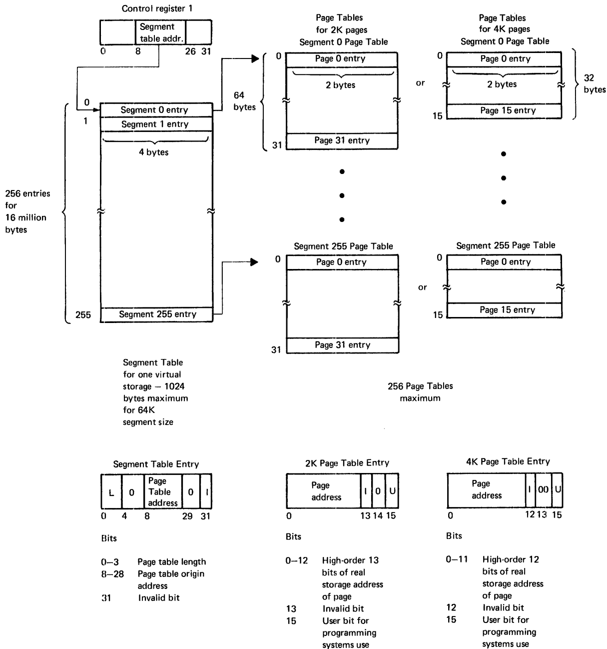
Figure 30.10.2. Segment table and page tables used for dynamic address translation
