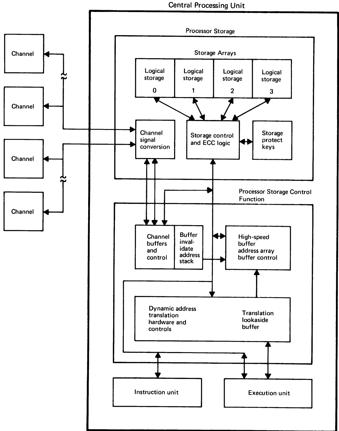
Figure 20.15.3. Model 168 components and controls
