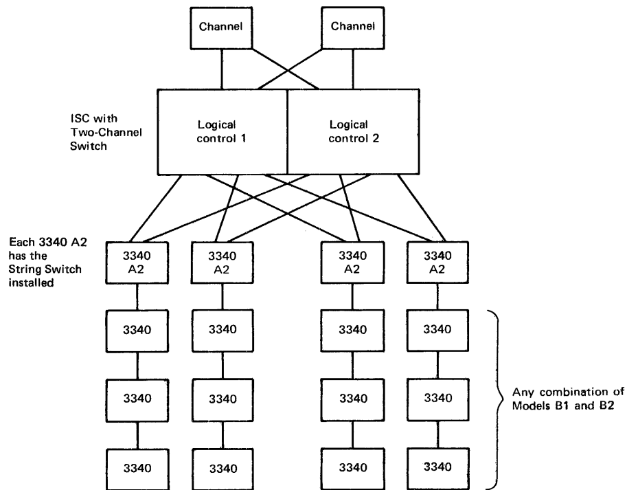
Figure 50.15.10. String switching for 3340 facilities attached to one ISC
